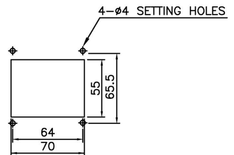
SETTING DIMENSION
